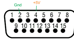
15 Dsub Male
