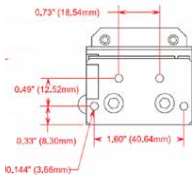
XSlide Assembly (End View)
